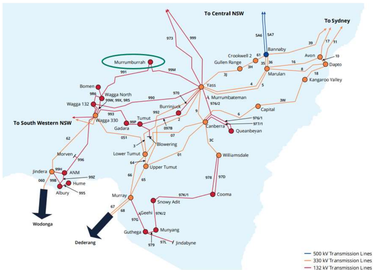
Figure 2-1 Location of Murrumburrah substation on the Southern NSW transmission network
