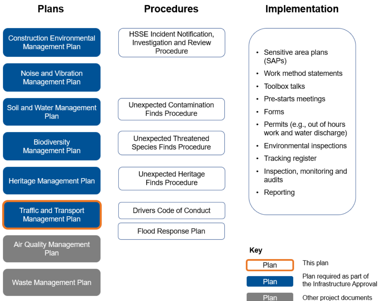
Figure 1.1 - CEMP framework
