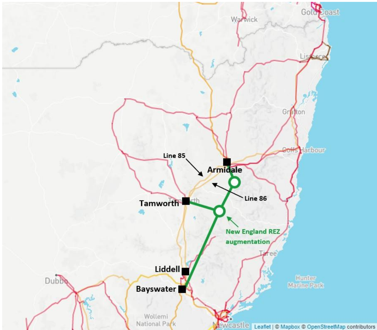
Figure 14: NNS network into NCEN 64
