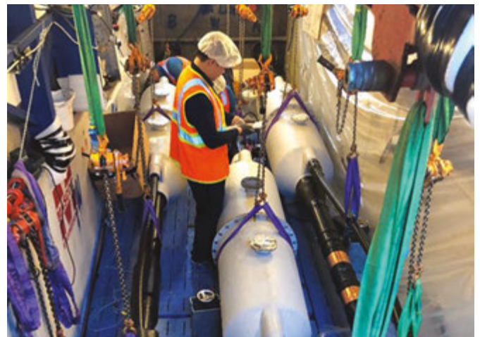
电缆接驳和调试 (Rawson Road接驳井, Greenacre)
